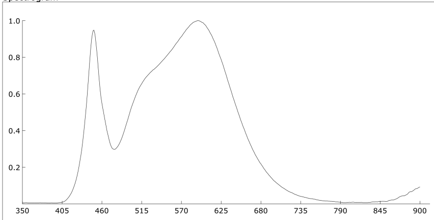
Spectrogram
